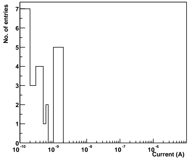
HV Leakage Current (@ 500V)
