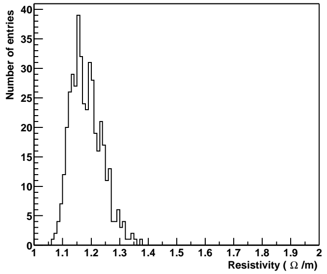
Resistivity of thin lines
