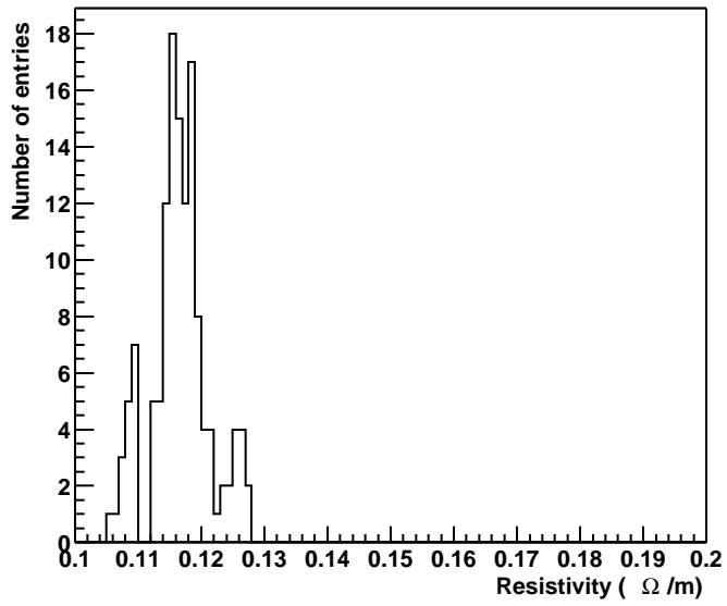
Resistivity of thick lines
