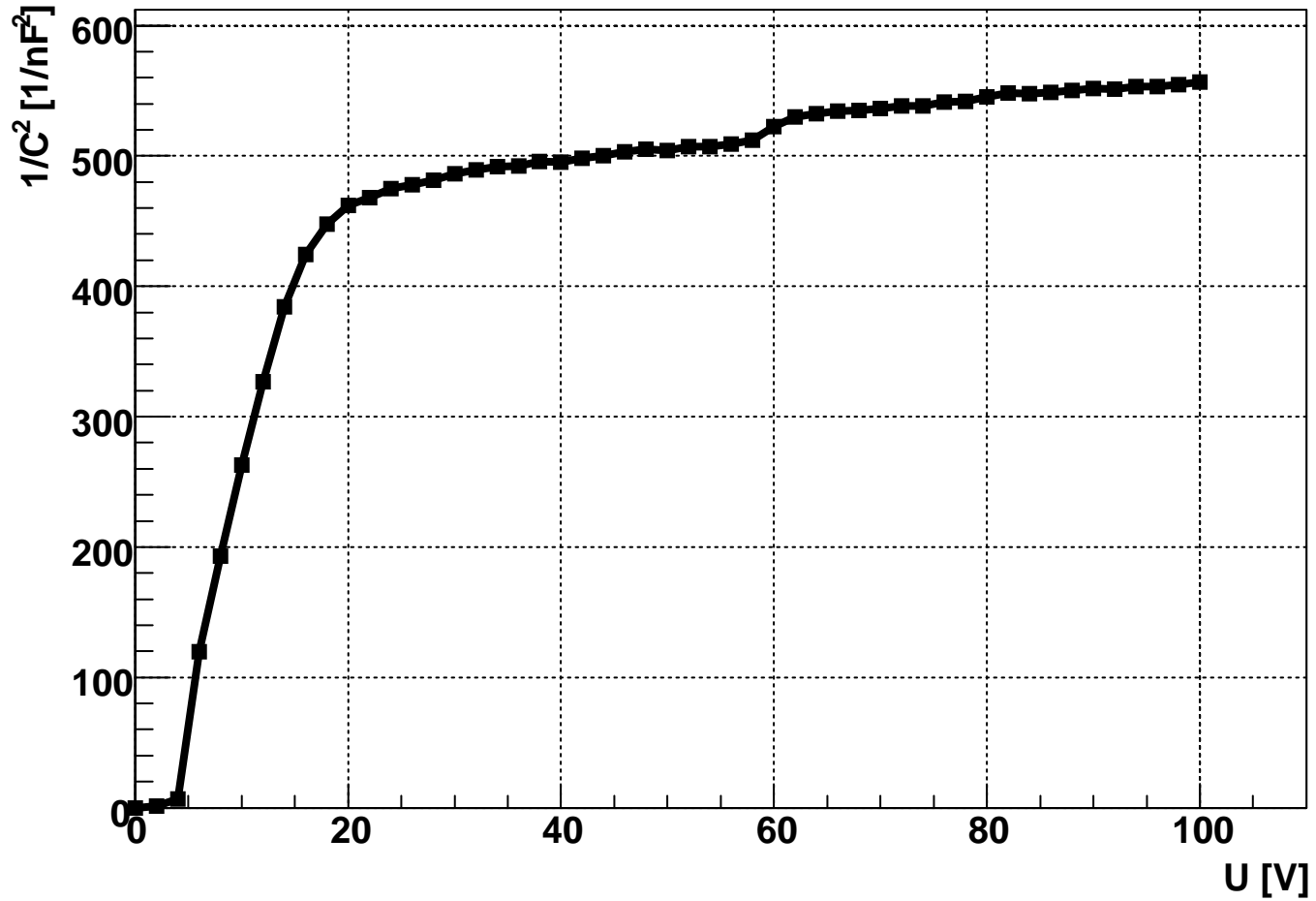
C-V measurement, f = 10 kHz
