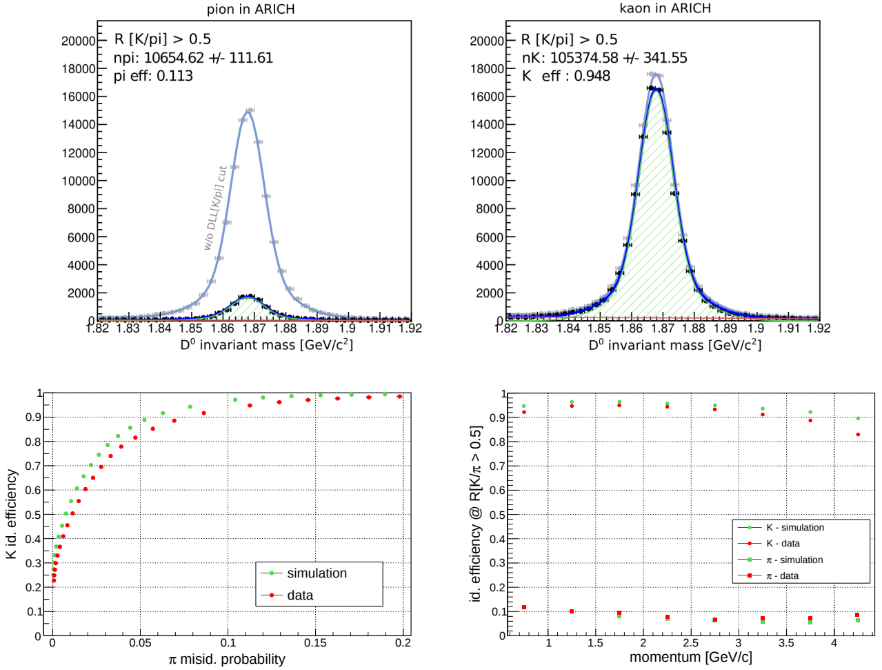
Figure 31: ARICH detector, performance. Top: examples of fits of the K^\mp\pi^\pm invariant mass distributions from which we determine kaon identification efficiency and pion misidentification probability at a given criterion on R[K/\pi] . Bottom left: kaon identification efficiency versus pion misidentification probability for all kaon/pion tracks from D^0 decays that enter the ARICH detector; right: kaon identification efficiency and pion misidentification probability as a function of track momentum for a fixed likelihood ratio, R[K/\pi] > 0.5 .
