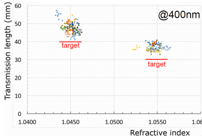
Figure 8: Aerogel properties of the installed tiles. The horizontal axis shows the refractive index, while the vertical axis shows the transmission length at 400 nm. Colours indicate different production batches.
