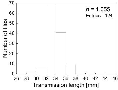
Figure 7: Aerogel properties of the installed tiles: the distribution over the transmission length at 400 nm for the upstream (top) and downstream tiles (bottom).
