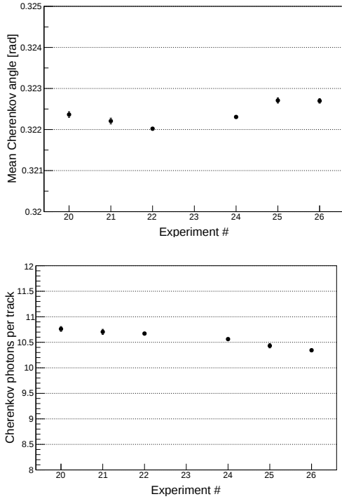
Figure 28: Detector performance as a function of time: Cherenkov angle (top) and number of photons (bottom) for ultra-relativistic muon tracks ( p > 4 GeV/c).
