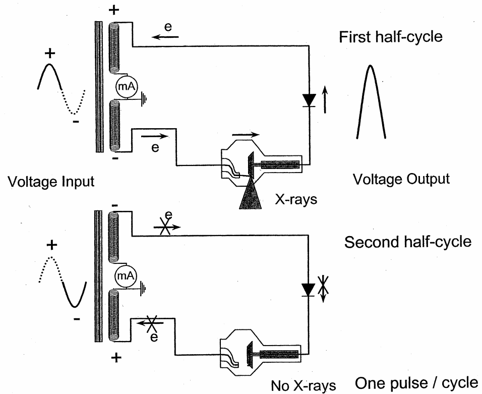
(a) Electron flow through single rectifier circuit
