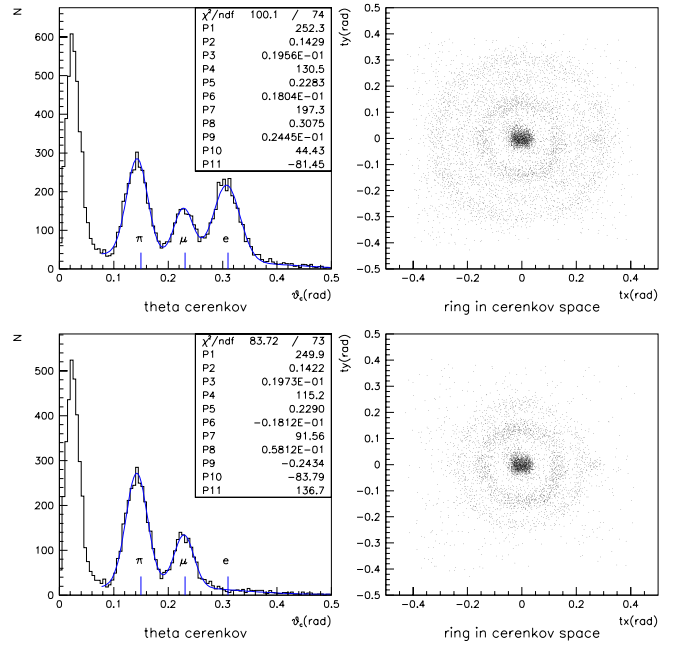
Fig. 3. Accumulated distributions of hits depending on their Cherenkov angle for all 0.8 GeV/c beam particles (top), and with gas Cherenkov signal vetoing the electrons (bottom).
