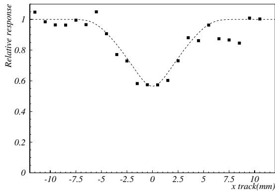
Fig. 7. The number of Cherenkov photons detected on the ring, as a function of the charged particle impact point distance from the side wall of the aerogel tile. The values shown are normalized to the measured values in case of a single tile covering the full range. Also shown is the estimate of a simple model.
