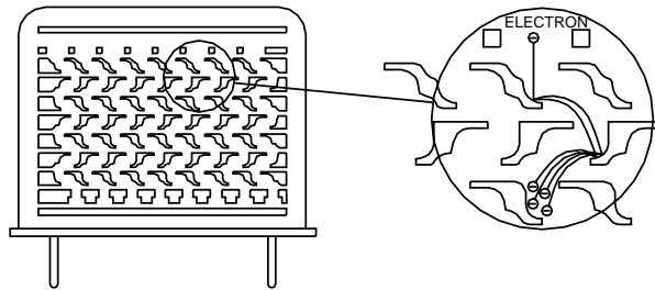
Figure 4: Metal channel type PMT [9].
