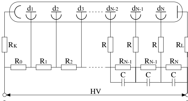
Figure 1: Voltage divider.
