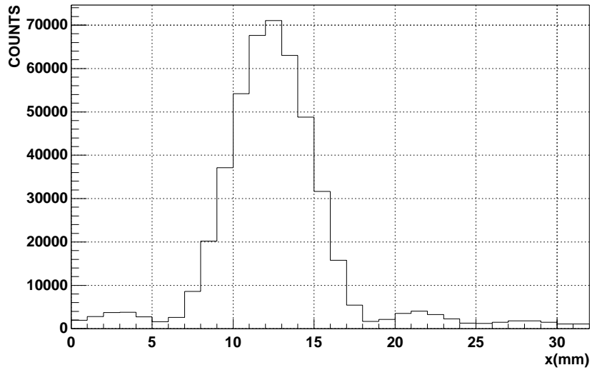
Figure 13: Measured diffraction distribution.
